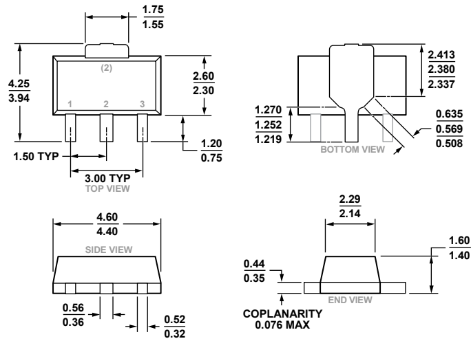
COMPLIANT TO JEDEC STANDARDS TO-243 Figure 33. 3-Lead Small Outline Transistor Package [SOT-89] (RK-3) Dimensions shown in millimeters
