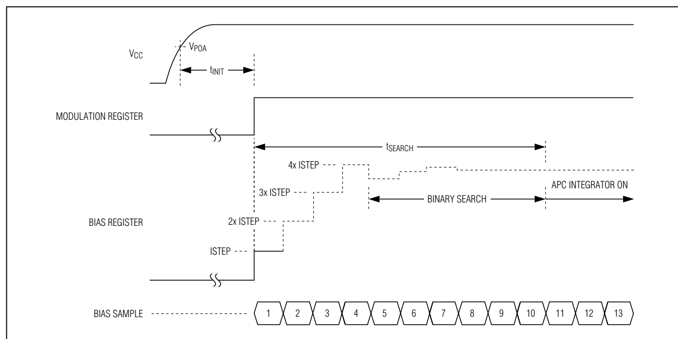
Figure 2. Power-Up Timing
