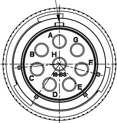
MASTER KEYWAY
