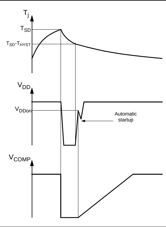
Figure 7. Thermal shutdown
