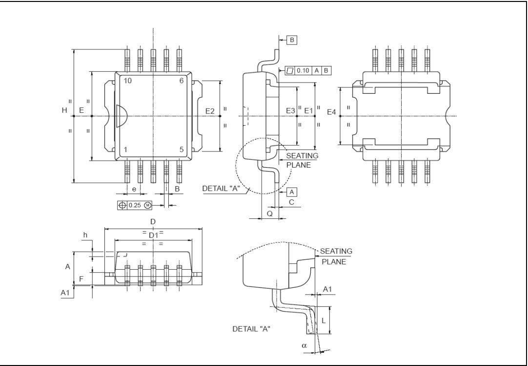
Figure 26. Package dimensions
