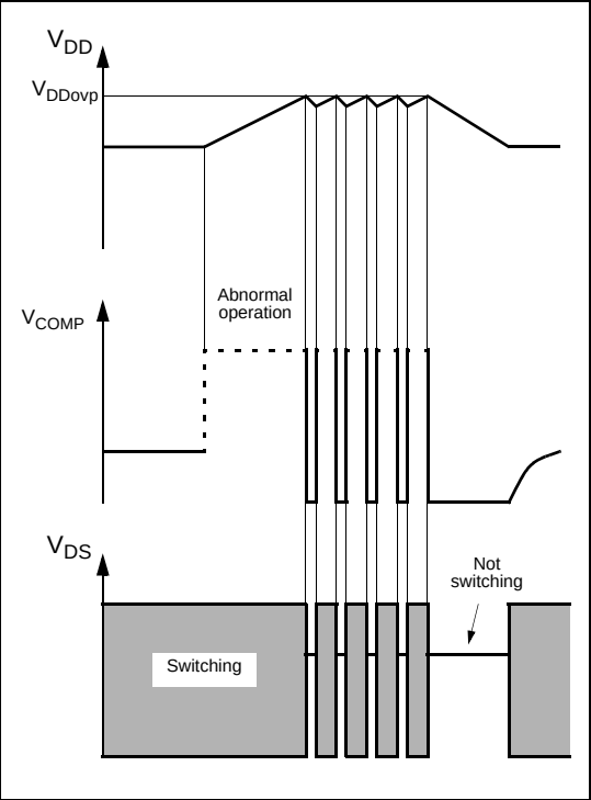
Figure 8. Overvoltage event
