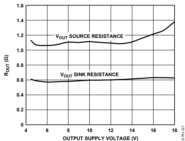
Figure 17. Typical Output Resistance ( R_{OUT} ) vs. Output Supply Voltage
