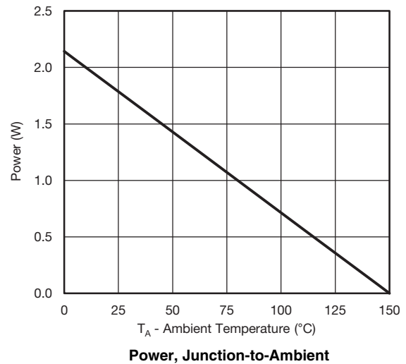
Power, Junction-to-Ambient
