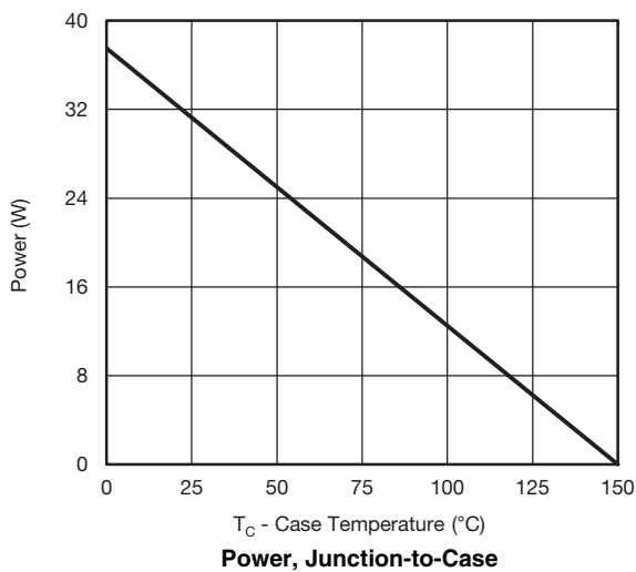
Power, Junction-to-Case
