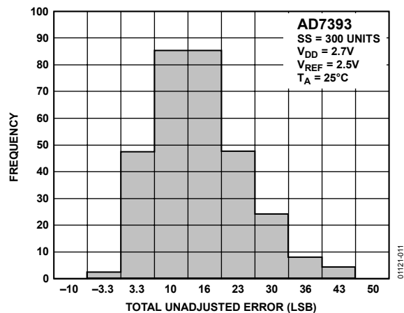
Figure 8. AD7393 Total Unadjusted Error Histogram
