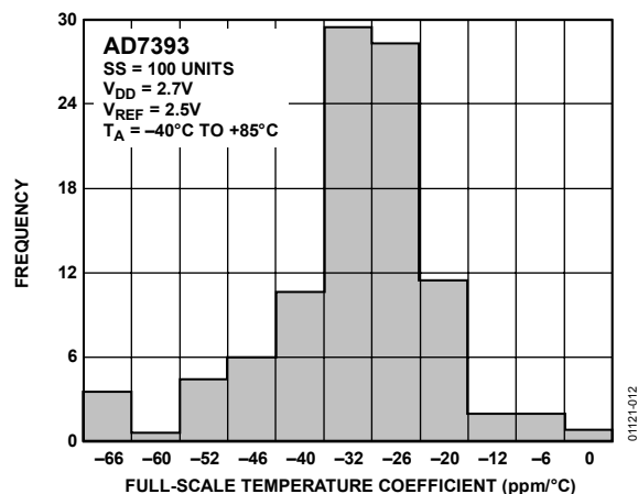
Figure 9. AD7393 Full-Scale Output Temperature Coefficient Histogram
