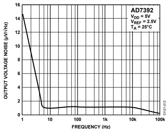
Figure 10. Voltage Noise Density vs. Frequency
