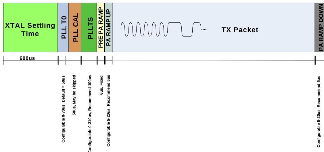
Figure 23.2. TX Timing
