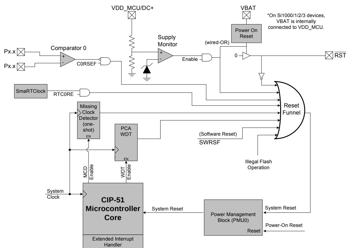
Figure 18.1. Reset Sources
