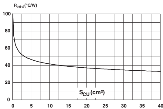
Figure 9. Junction to ambient thermal resistance versus copper surface under tab, PCB FR4, copper thickness 35μm
