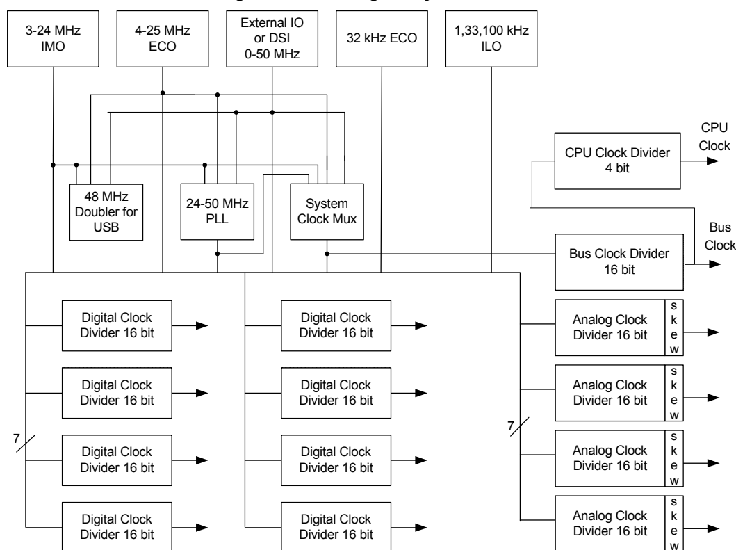
Figure 6-1. Clocking Subsystem
