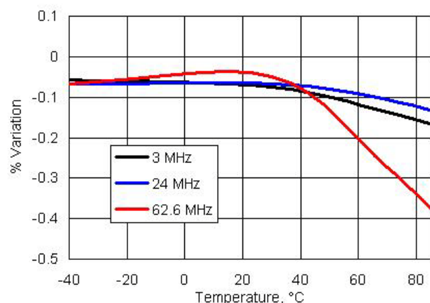
Figure 11-58. IMO Frequency Variation vs. Temperature
