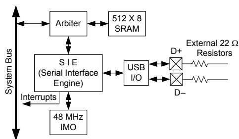
Figure 7-18. USB
