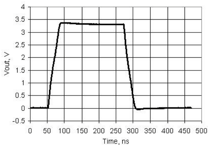
Figure 11-16. GPIO Output Rise and Fall Times, Slow Strong Mode, V_{DDIO} = 3.3 V, 25 pF Load
