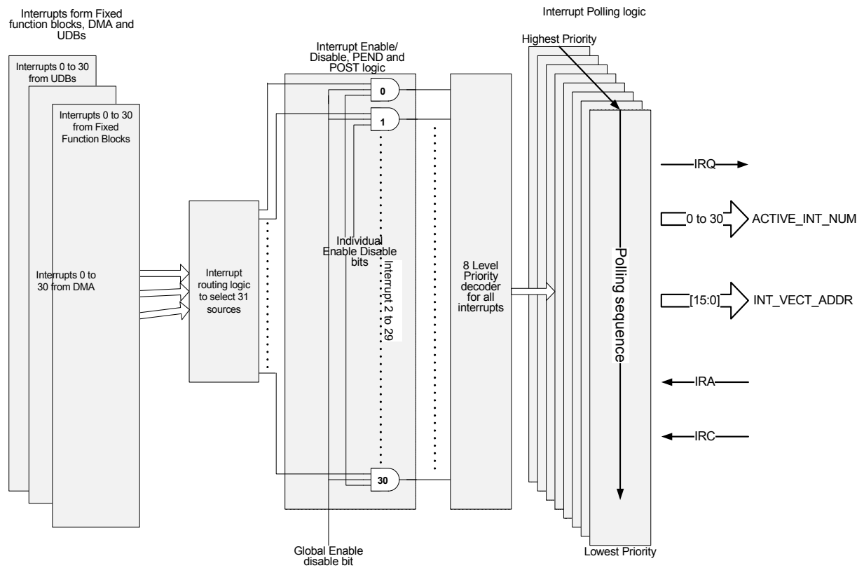
Figure 4-3. Interrupt Structure
