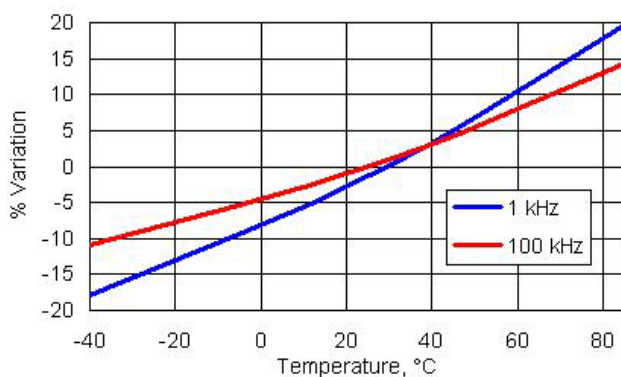
Figure 11-60. ILO Frequency Variation vs. Temperature
