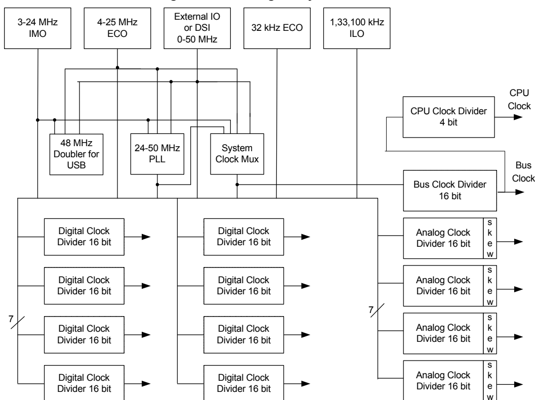
Figure 6-1. Clocking Subsystem
