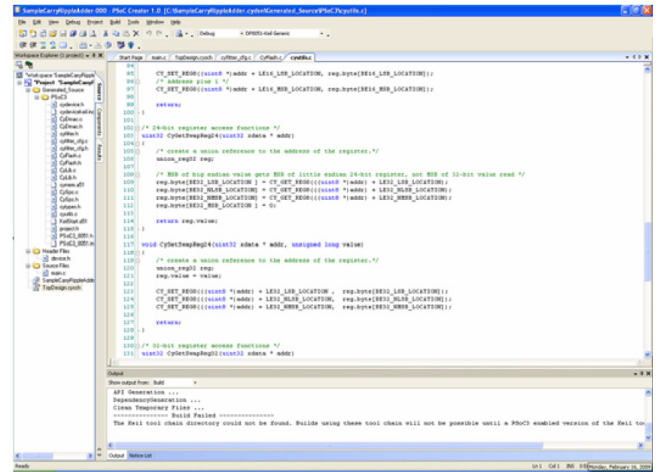
Figure 7-4. Code Editor
