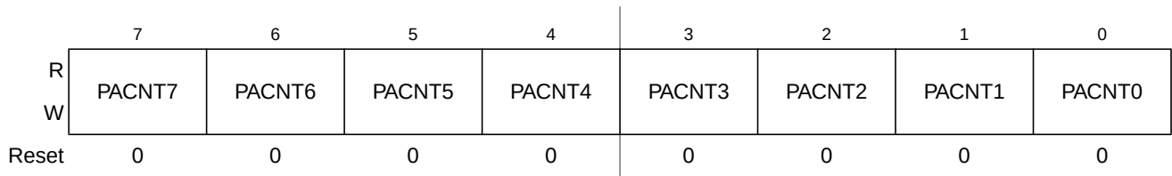
Figure 16-27. Pulse Accumulator Count Register Low (PACNTL)
