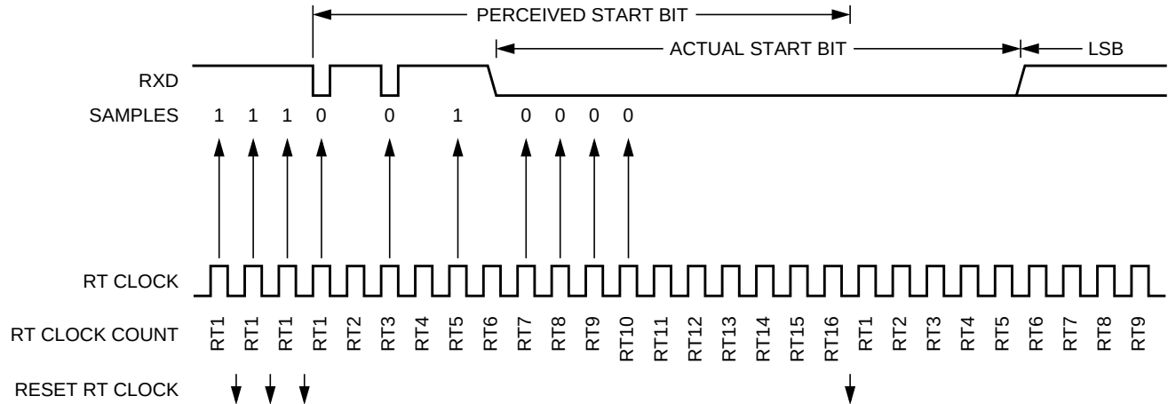
Figure 13-18. Start Bit Search Example 3
