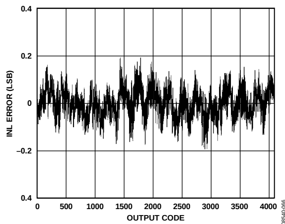
Figure 14. INL with f_{IN} = 9.7 MHz
