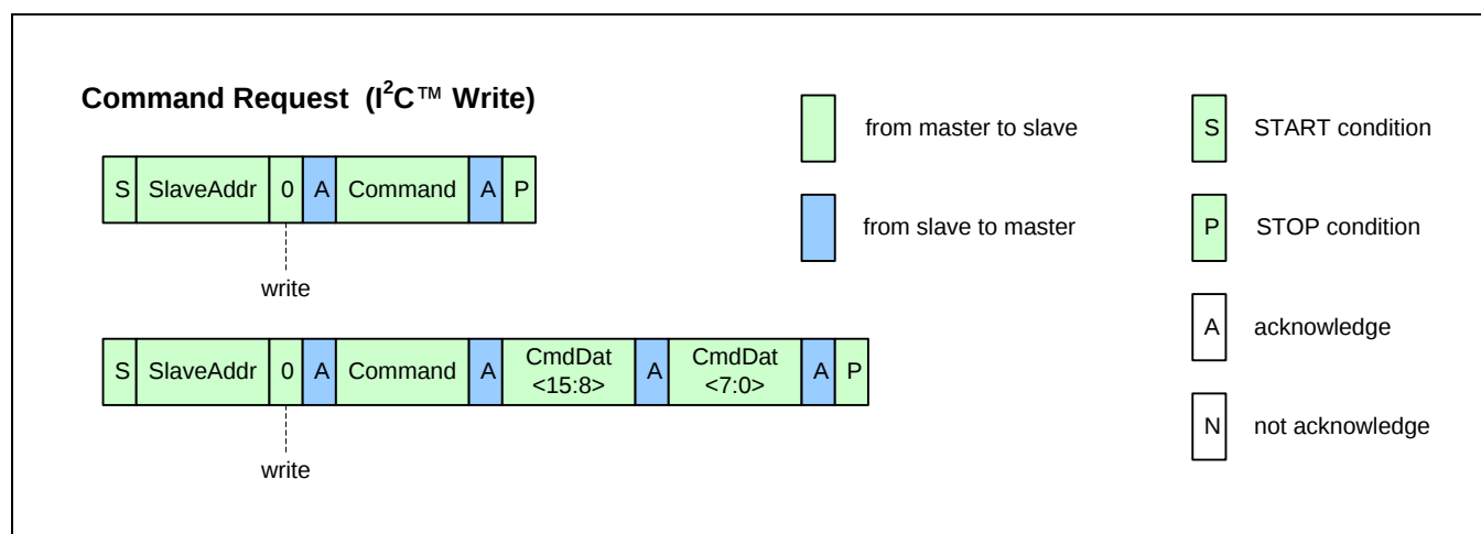
Figure 3.8 I 2 C™ Command Request
