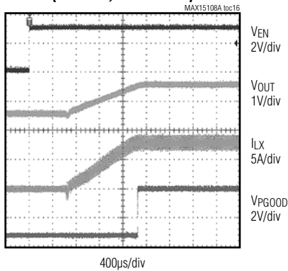
ENABLE INTO PREBIASED 0.5V OUTPUT (8A LOAD, PWM MODE)
