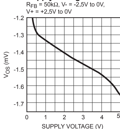
Offset Voltage vs. Supply Voltage R_{FB} = 50\text{k}\Omega , V_- = -2.5\text{V} to 0\text{V} , V_+ = +2.5\text{V} to 0\text{V}
