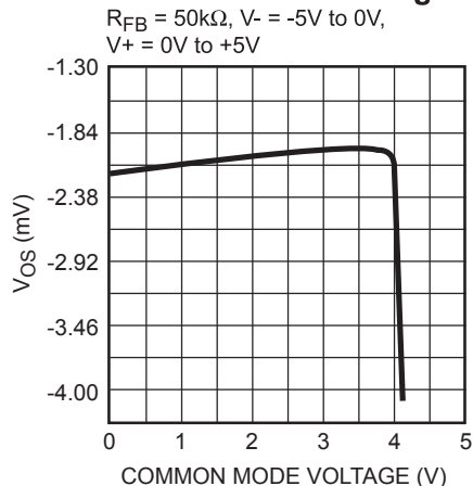
Offset Voltage vs. Common Mode Voltage R_{FB} = 50\text{k}\Omega , V_- = -5\text{V} to 0\text{V} , V_+ = 0\text{V} to +5\text{V}
