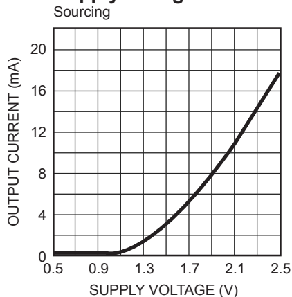
Short Circuit Current vs Supply Voltage Sourcing
