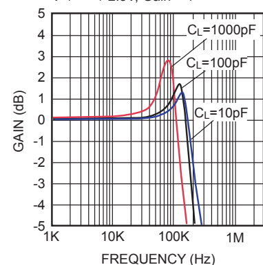
Close-Loop Unity Gain Frequency Response
