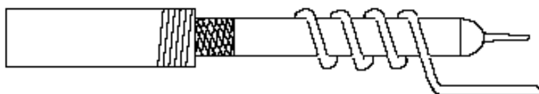
Figure – 6 : Low-loop-inductance Oscilloscope Probe
