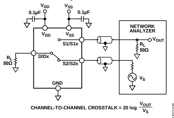
Figure 40. Channel-to-Channel Crosstalk
