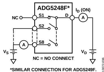
Figure 37. On Leakage
