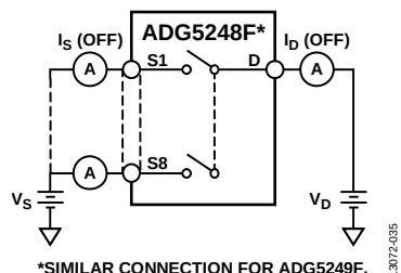
Figure 36. Off Leakage
