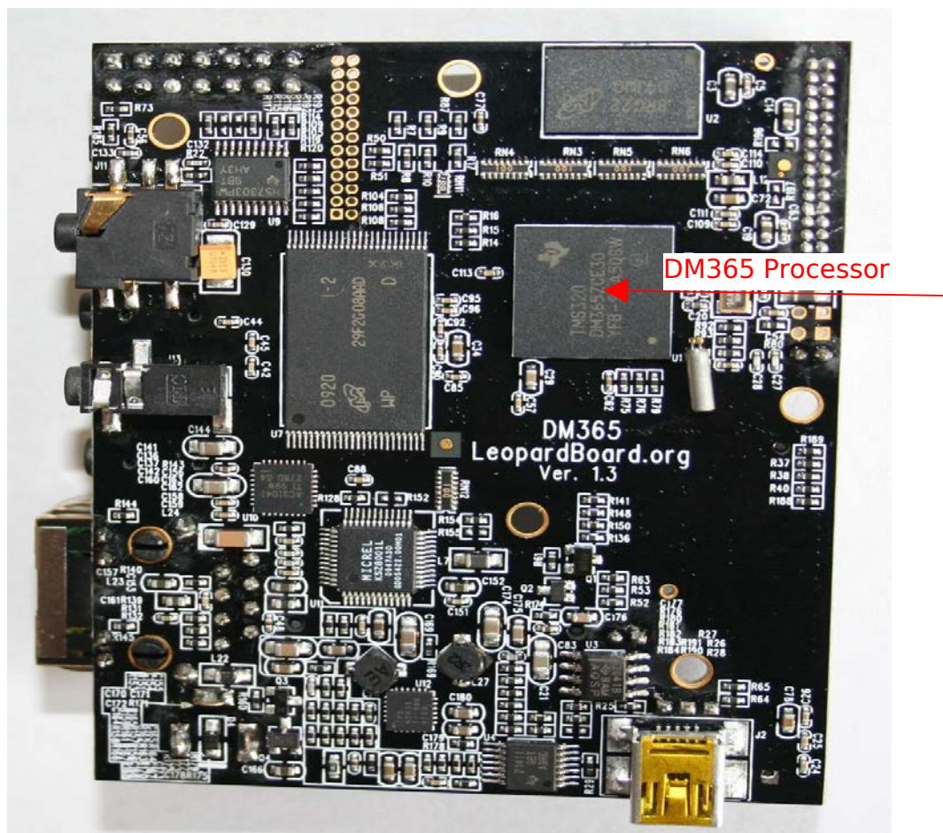
Figure 23. DM355 Processor
