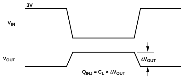
Figure 18. Charge Injection
