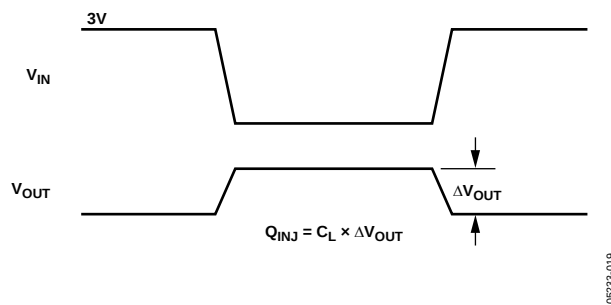
Figure 18. Charge Injection
