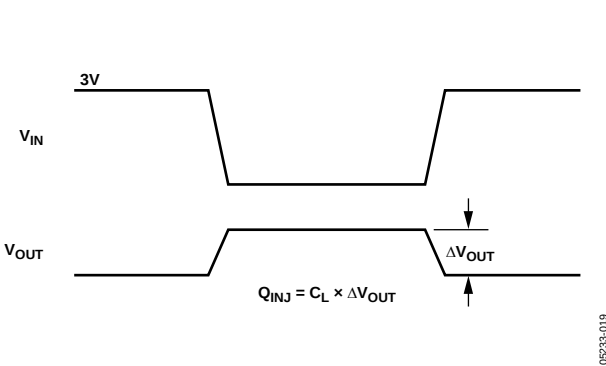
Figure 18. Charge Injection
