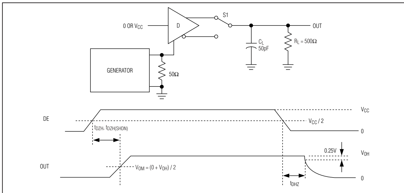
Figure 4. Driver Enable and Disable Times ( t_{DZH} , t_{DZH(SHDN)} )
