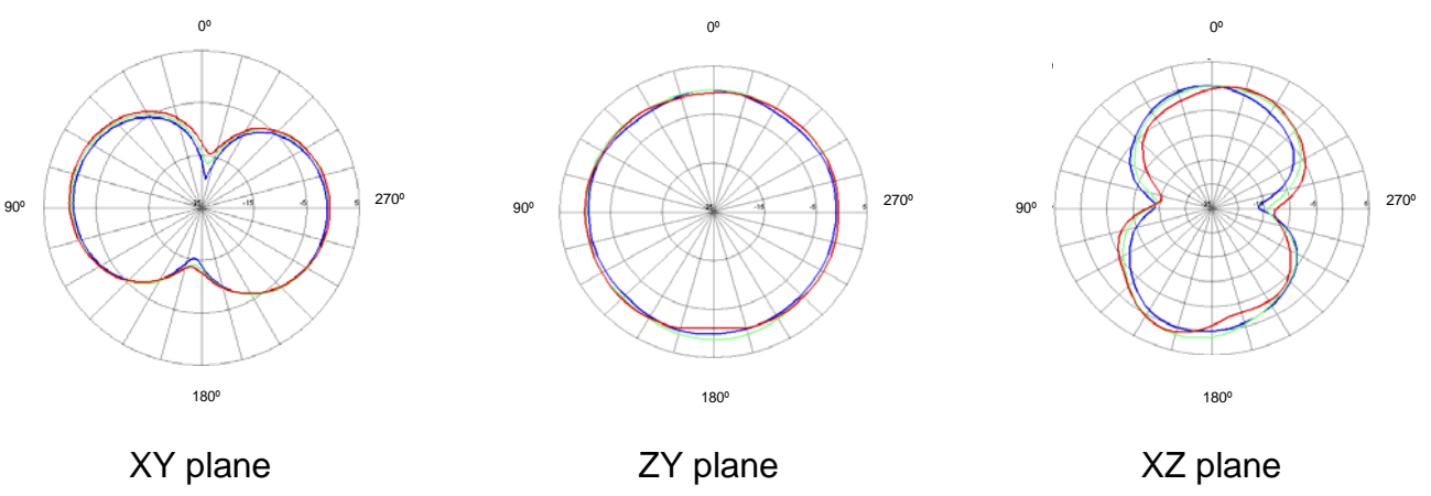
Patterns show combined polarisations measured on reference board A10376-U1. 3D Pattern measured at 890MHz
