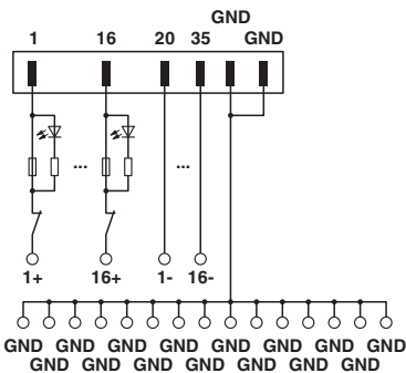
Circuit diagram
