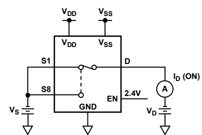
Figure 21. I_D (On)
