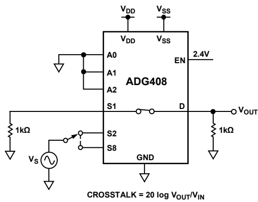
Figure 27. Channel-to-Channel Crosstalk
