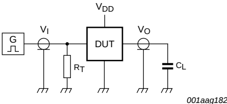
Test data given in Table 10 . Definitions for test circuit: DUT = Device Under Test. C_L = load capacitance including jig and probe capacitance. R_T = termination resistance should be equal to the output impedance Z_o of the pulse generator.
