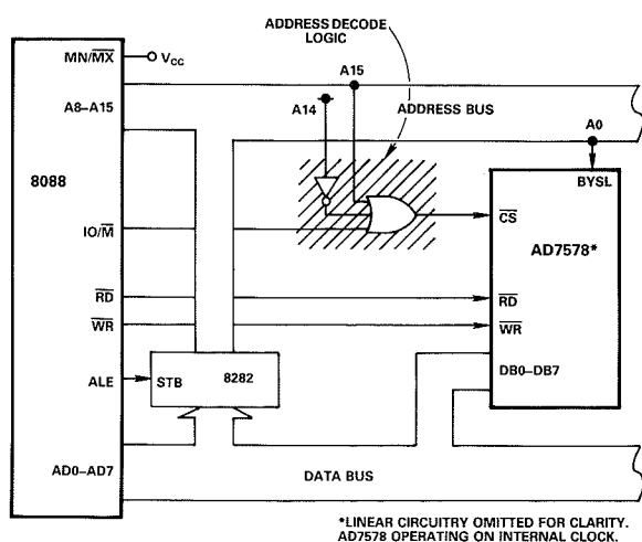
Figure 21. AD7578 – 8088 Interface
