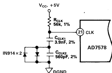
Figure 6. Circuitry Required for Internal Clock Operation
