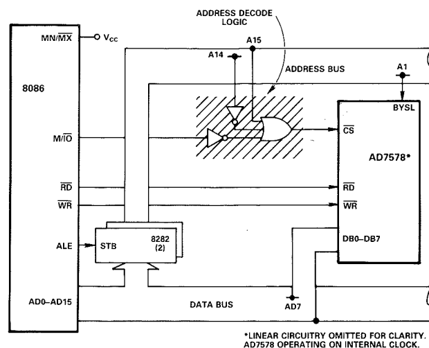
Figure 22. AD7578 – 8086 Interface
