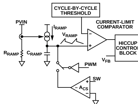
Figure 35. Current-Limit Circuit
