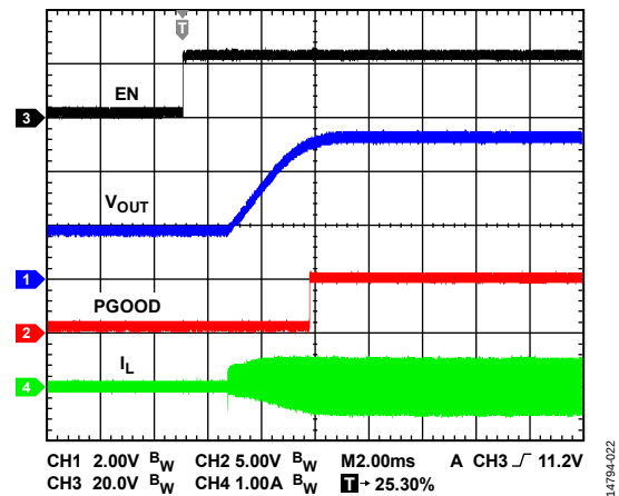
Figure 22. Voltage Precharged Output
