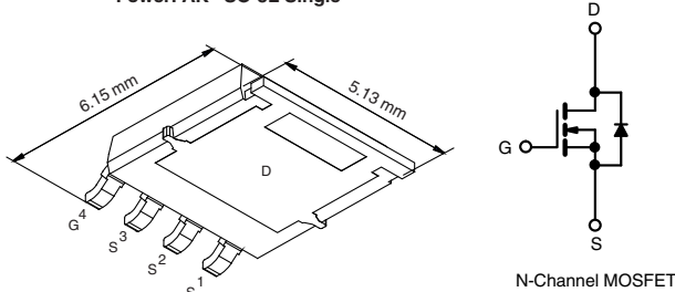
N-Channel MOSFET
