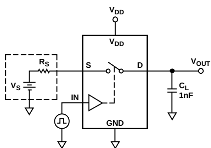
Figure 15. Charge Injection
