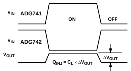
Figure 15. Charge Injection
