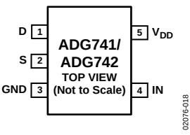
Figure 4. 5-Lead Pin Configuration
