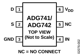
Figure 3. 6-Lead Pin Configuration
