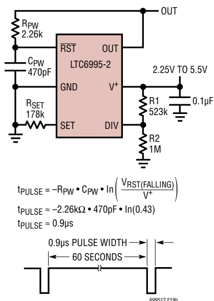
Figure 19b. Self-Resetting Circuit (DIVCODE = 10)
