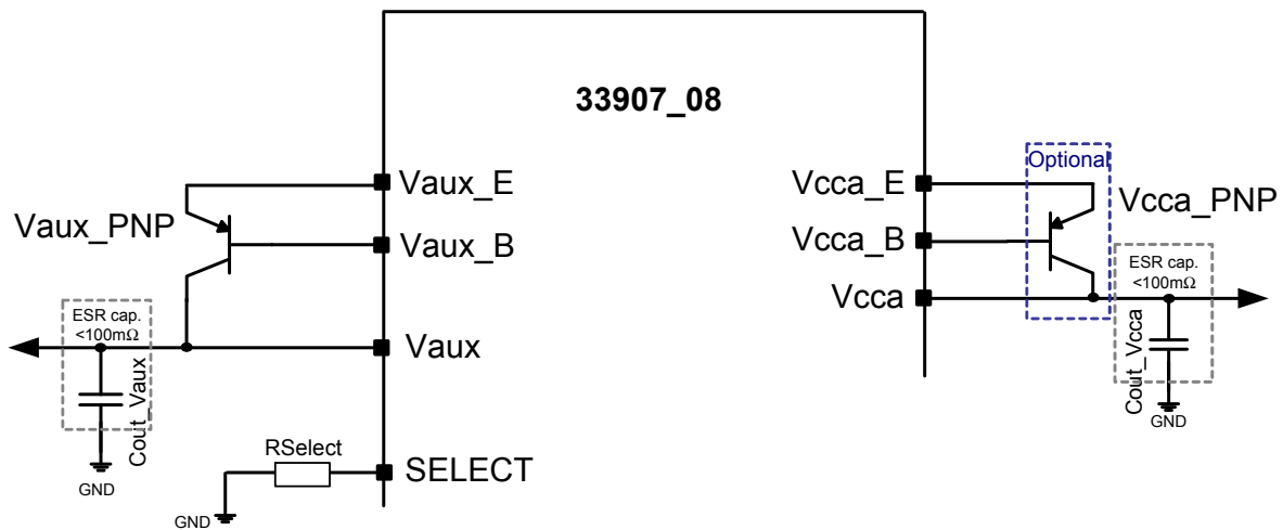
Figure 35. Vaux/Vcca Connection
