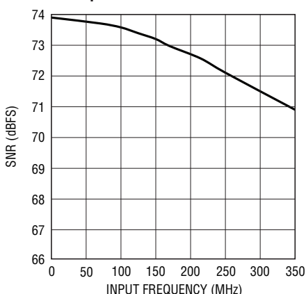
LTC2258-14: SNR vs Input Frequency, -1\text{dB} , 2\text{V} Range, 65\text{Mps}
