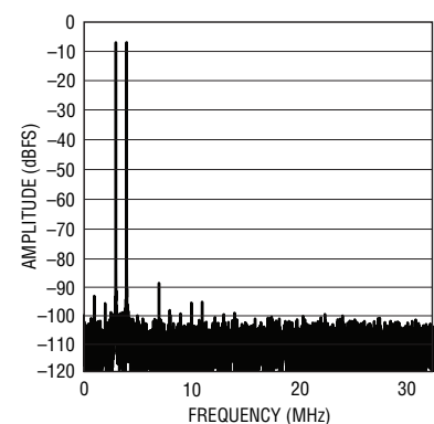
LTC2258-14 2-Tone FFT, f_{IN} = 68MHz and 69MHz
