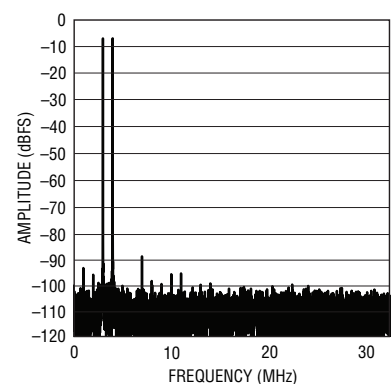
LTC2258-14 2-Tone FFT, f IN = 68MHz and 69MHz
