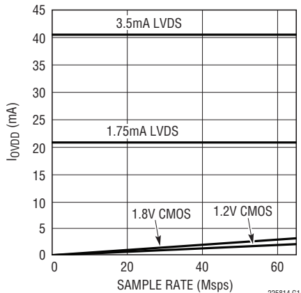
LTC2258-14: I_{OVPD} vs Sample Rate, 5MHz Sine Wave Input, -1dB, 5pF on Each Data Output
