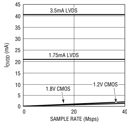
LTC2257-14: I_{OVPD} vs Sample Rate, 5\text{MHz} Sine Wave Input, -1\text{dB} , 5\text{pF} on Each Data Output
