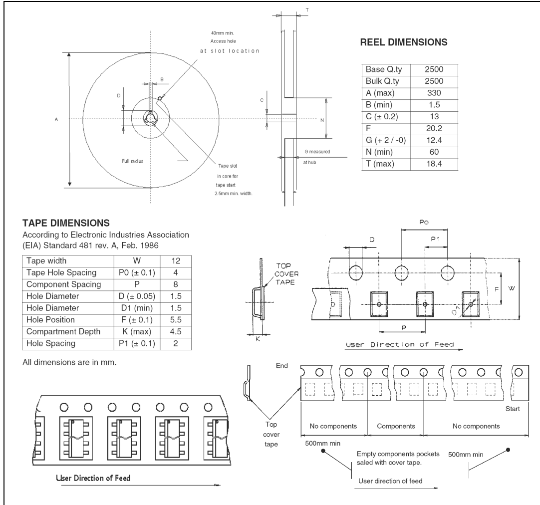
Figure 17. PowerSSO-12™ tape and reel shipment (suffix “TR”)
