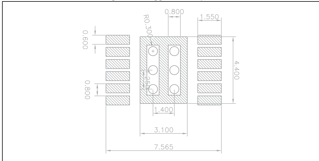
Figure 18. Suggested footprint
