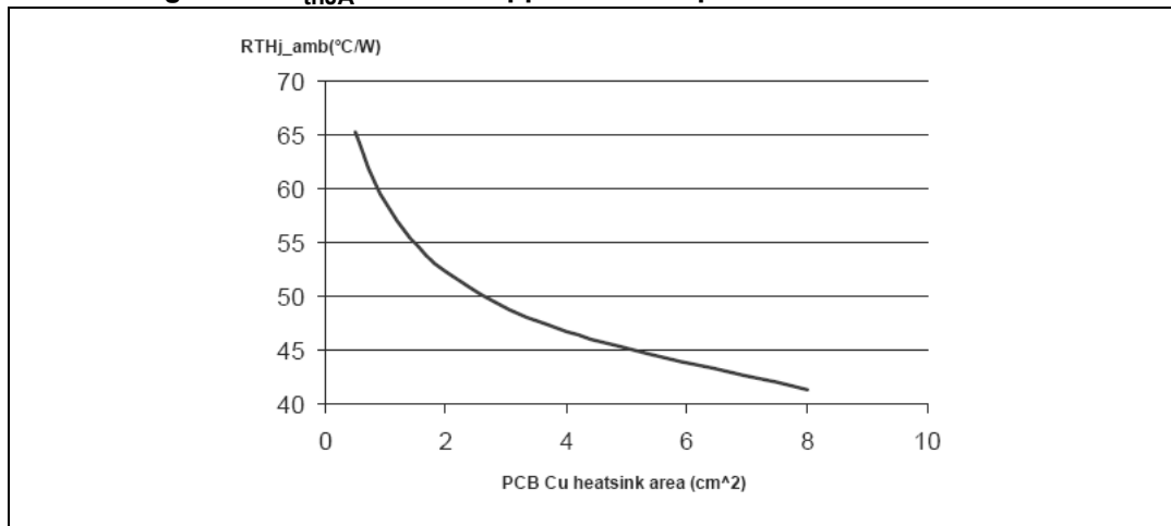
Figure 11. R_{thJA} vs PCB copper area in open box free air condition
