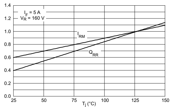
Figure 10. Dynamic parameters versus junction temperature (reference: T_i = 125\text{ °C} )
