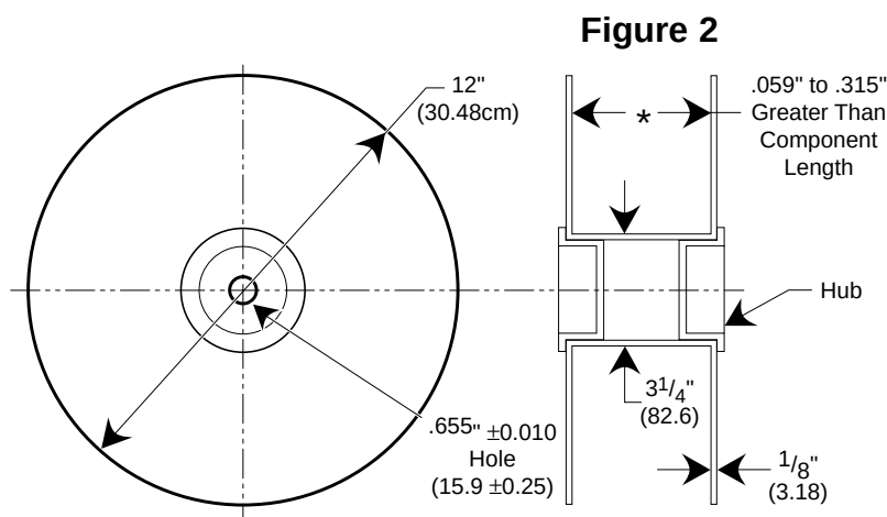
COMPONENT BODY DIAMETER COMPONENT PITCH "A" INSIDE TAPE SPACING "B" ±1.5mm (0.059") 0.020" or (±0.5mm) I II III 0" (0mm) to 0.197" (5mm) 0.200" or (5mm) 2.062" 2.500" 2.874" 0.197" (5.01mm) to 0.394" (10mm) 0.400" or (10mm) (52.4mm) (63.5mm) (73mm)
