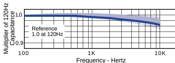
Figure 1. Normal Effect of Frequency upon Capacitance
