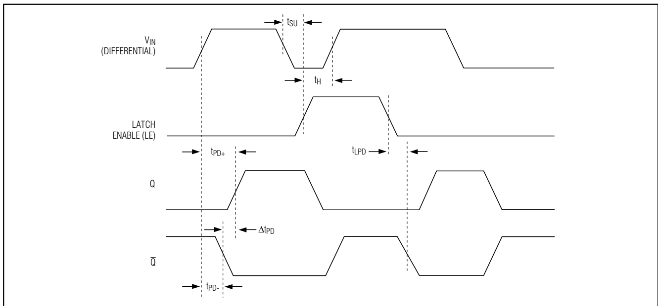
Figure 1. Timing Diagram
