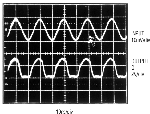
MAX912/MAX913 RESPONSE TO 50MHZ ( \pm 10mV_{p-p} ) SINE WAVE
