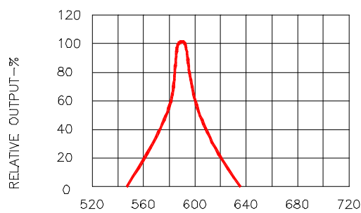
Fig.2 SPECTRAL RESPONSE
